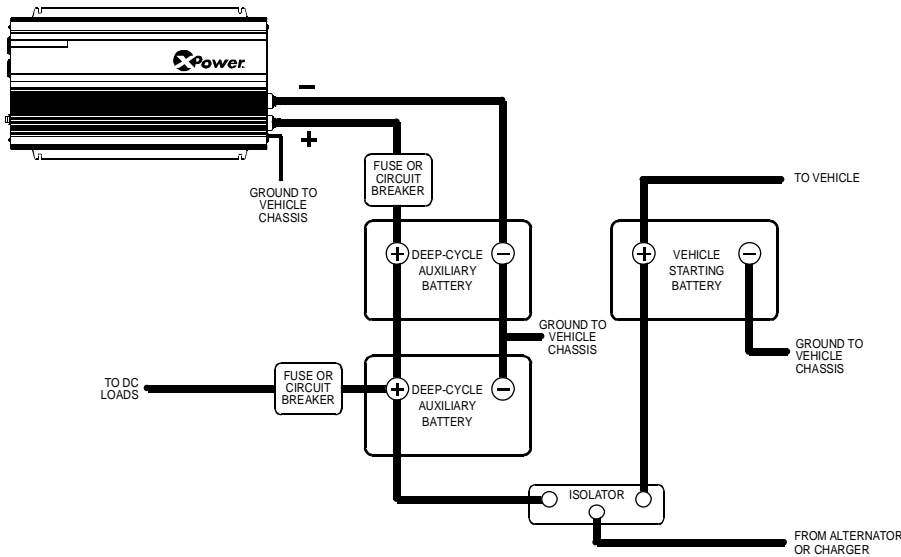
Figure 3-1 Configuration for Normal Loads
