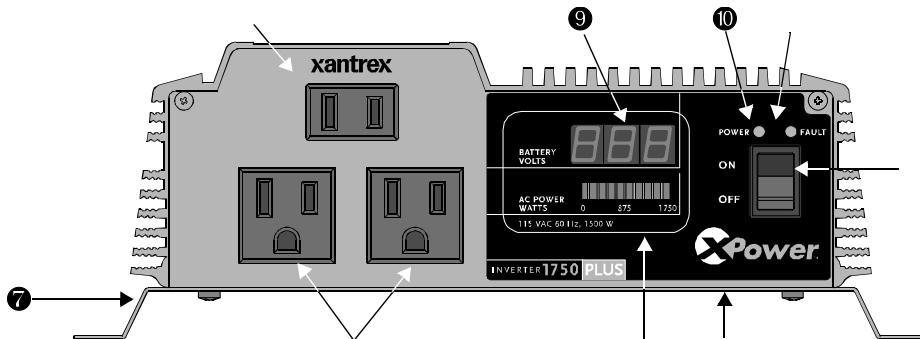
Figure 2-1 AC Panel (XPower 1750 Plus shown)
