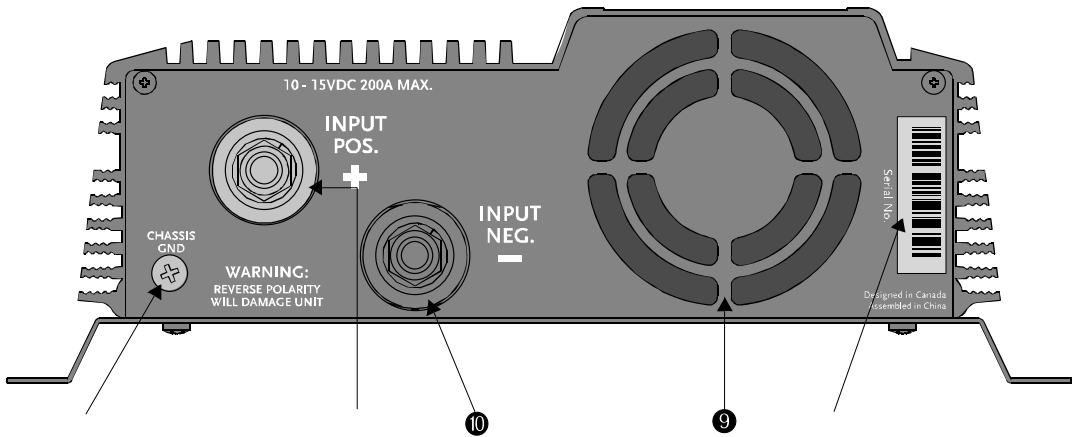
Figure 2-2 DC Panel (XPower 1750 Plus shown)
